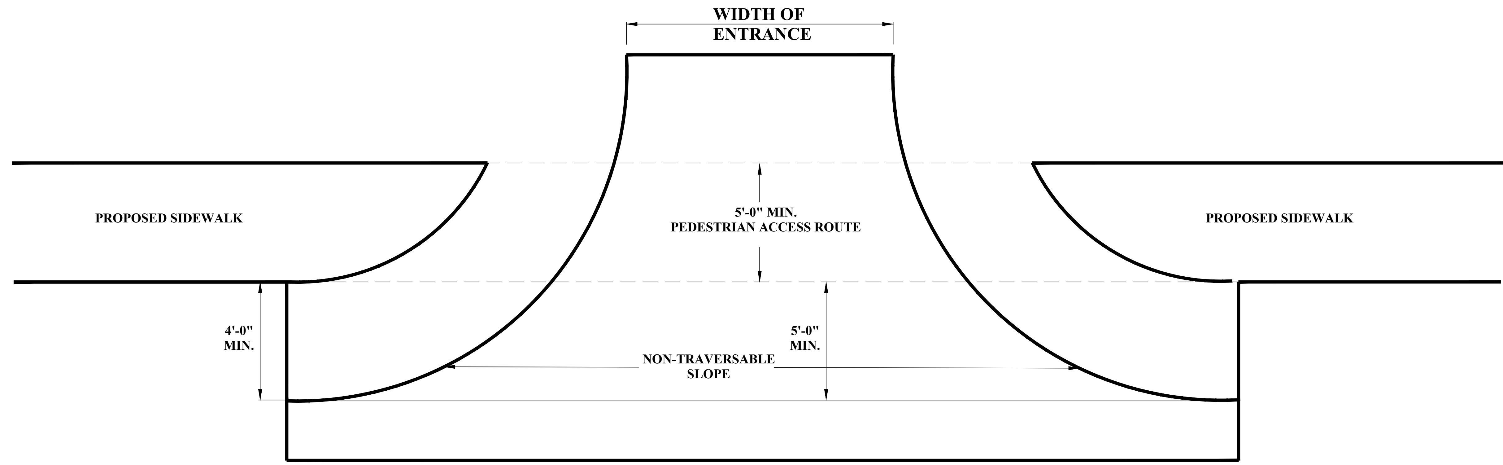
ENTRANCE TYPICAL (NOT TO SCALE)
