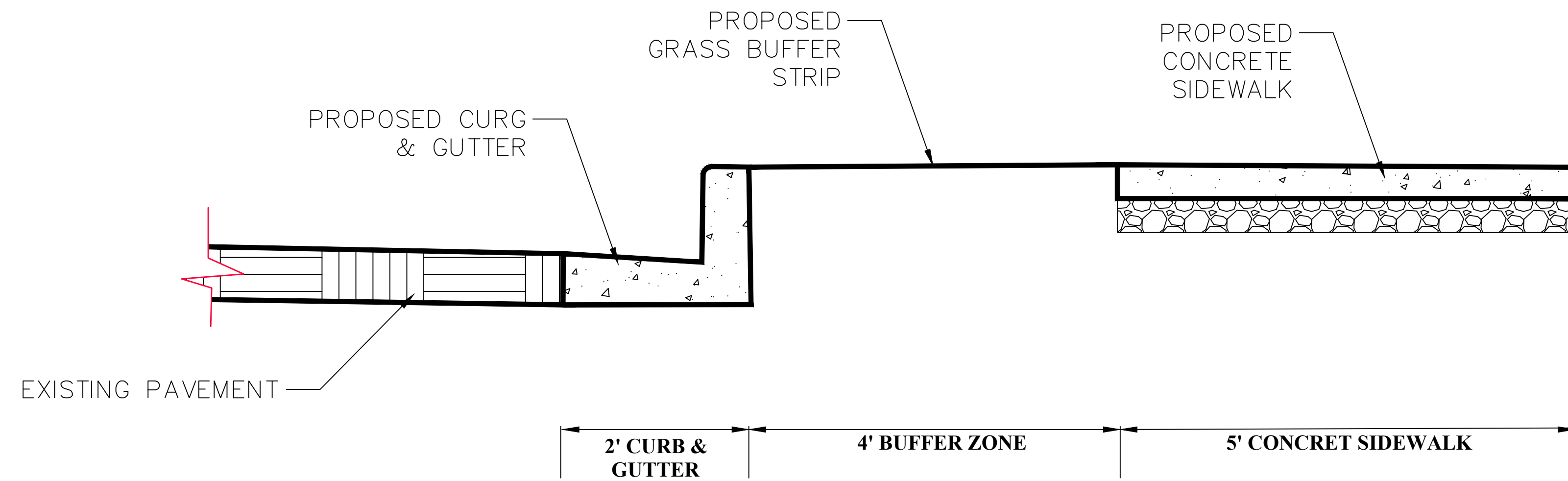
SIDEWALK TYPICAL (NOT TO SCALE)
